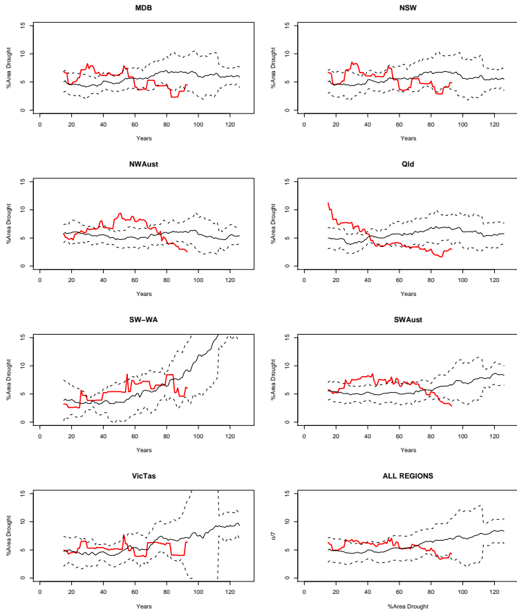
Figure 1: The 30 year moving average of area of exceptionally low rainfall observations (red) and average of 13 model results (black, with one standard deviation dashed). The results are presented for each region, and all regions combined.
