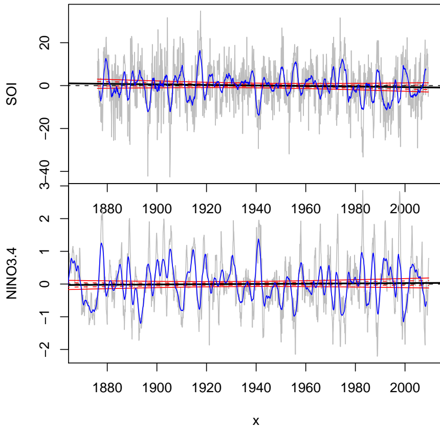
Figure 1: The trend in the SOI (upper) and NINO3.4 (lower), 95% confidence intervals without autocorrelation (red dashed) and with autocorrelation (red solid) and the 24 month moving average (blue).
